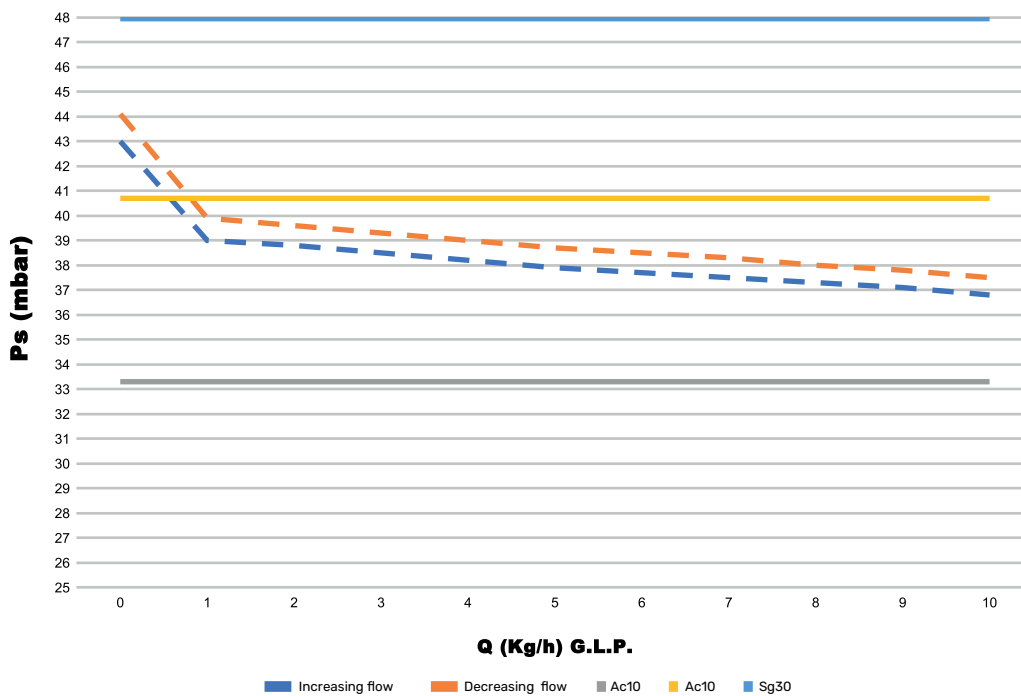
Pe: 200mbar
