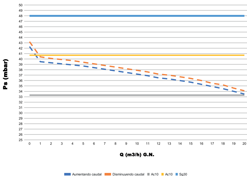
Pe: 1bar (Ps: regulada a 37mbar)
